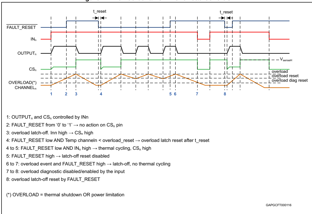
Figure 12. Device behavior in overload condition
