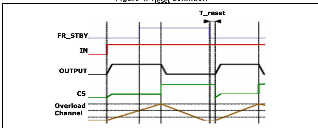
Figure 4. T_{reset} definition
