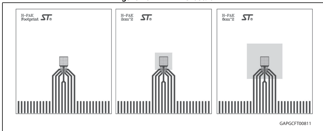
Figure 26. HPAK PC board
