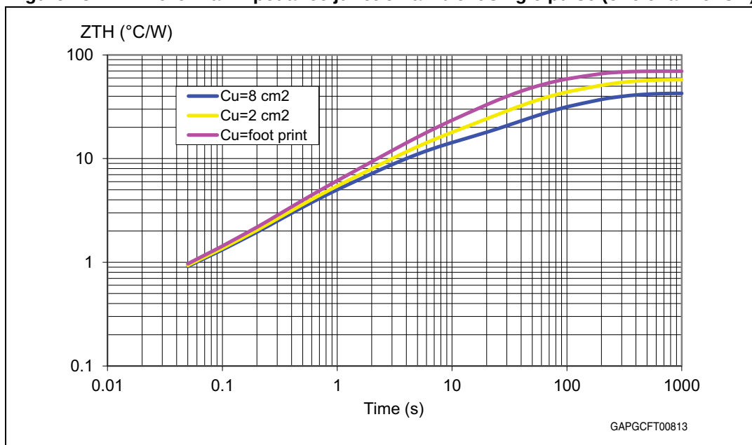
Figure 28. HPAK thermal impedance junction ambient single pulse (one channel ON)
