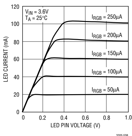
Figure 8. Compliance Voltage Required to get Higher LED Currents
