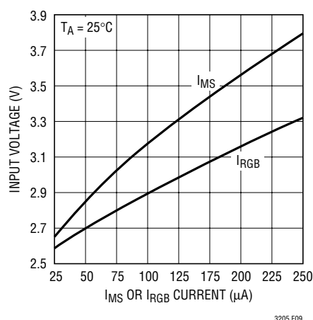
Figure 9. Input Supply Voltage Required to Support Higher Currents
