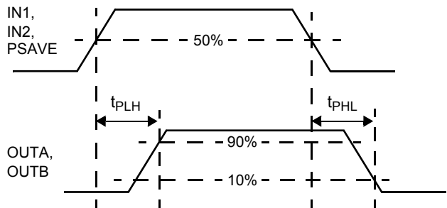
Figure 4. t_{PLH} and t_{PHL} Timing
