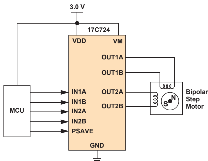
Figure 1. 17C724 Simplified Application Diagram
