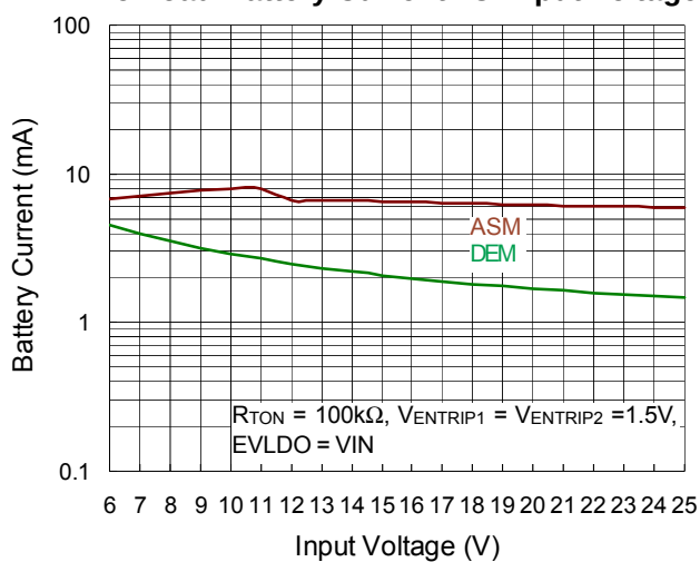
No Load Battery Current vs. Input Voltage
