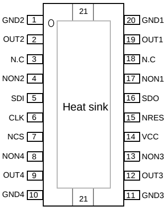
Figure 3. 33385 Pin Connections
