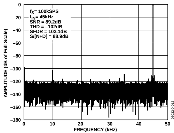
Figure 12. FFT Plot
