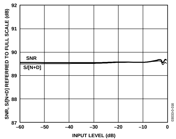
Figure 16. SNR and S/(\text{N}+\text{D}) vs. Input Level (Referred to Full Scale)
