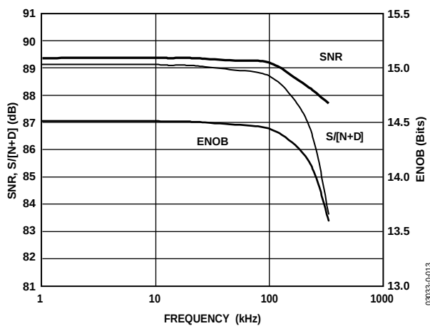
Figure 13. SNR, S/(\text{N}+\text{D}) , and ENOB vs. Frequency
