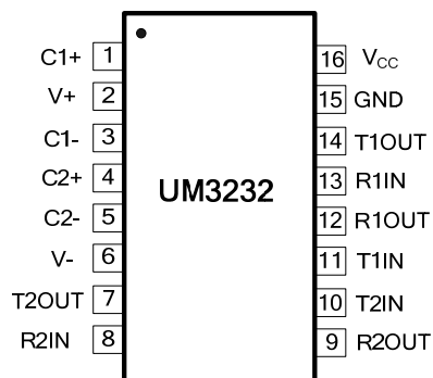
SOP16/DIP16/TSSOP16/SSOP16
