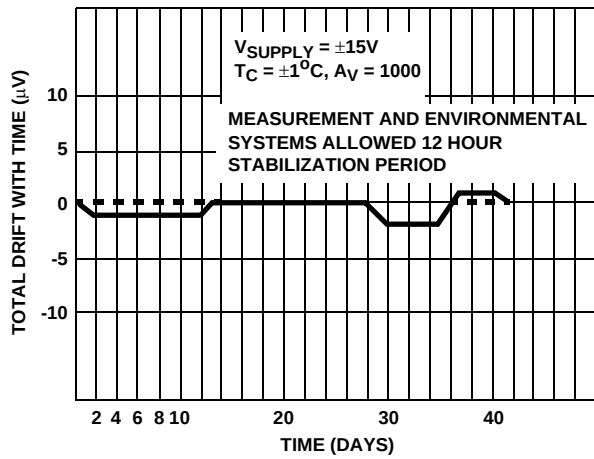
FIGURE 9. HA-5135 OFFSET VOLTAGE STABILITY vs TIME
