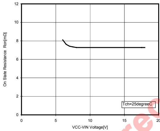
ON STATE RESISTANCE VS. VCC - VIN VOLTAGE
