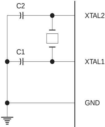
Figure 7. Oscillator Connections
