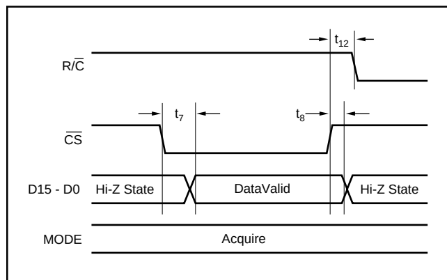
FIGURE 3. Bus Timing.
