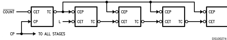
FIGURE 2. Multistage Counter with Lookahead Carry
