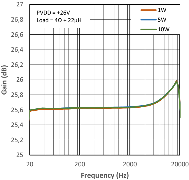
Figure 10-28 Gain vs Frequency for PMP4
