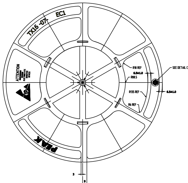
VIEW B
