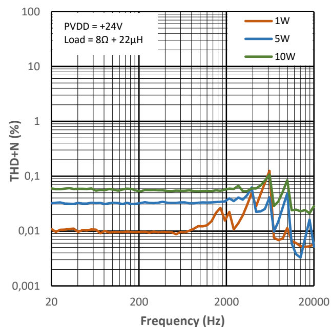
Figure 13-8 THD+N vs Frequency for PMP4
