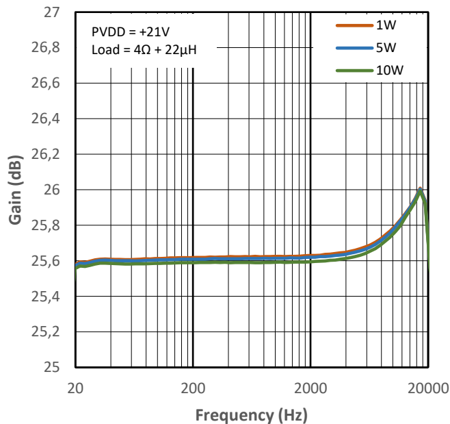
Figure 14-23 Gain vs Frequency for PMP2
