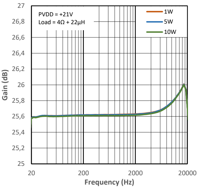
Figure 14-22 Gain vs Frequency for PMP1
