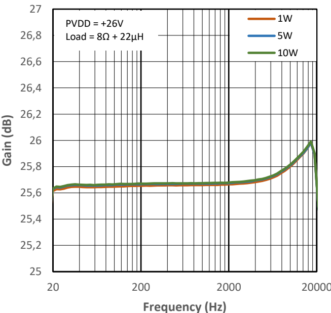
Figure 11-28 Gain vs Frequency for PMP4
