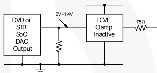
Figure 10. DC-coupled Inputs and Outputs
