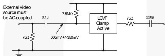
Figure 15. Biased SCART with AC-Coupled Outputs
