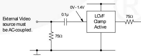
Figure 12. SCART with DC-coupled Outputs
