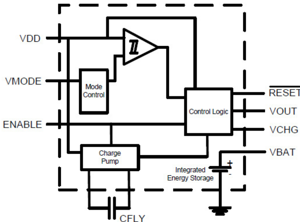
Figure 2: EnerChip CC CBC3105 Internal Block Diagram
