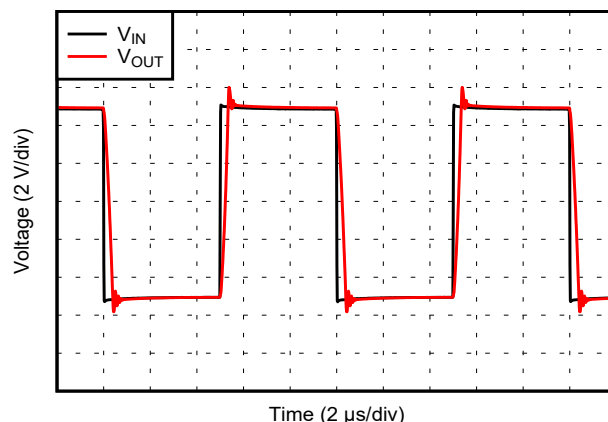
Figure 6-56. Small-Signal Step Response
