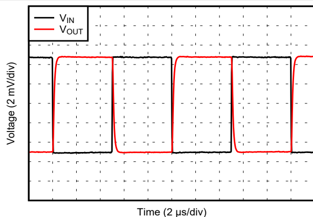
Figure 6-55. Small-Signal Step Response
