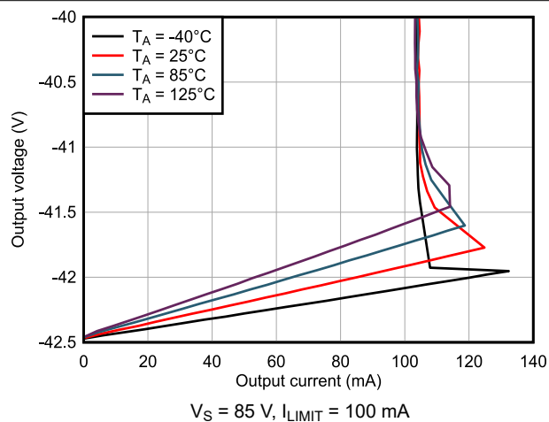
Figure 6-24. Output Voltage vs Output Sinking Current
