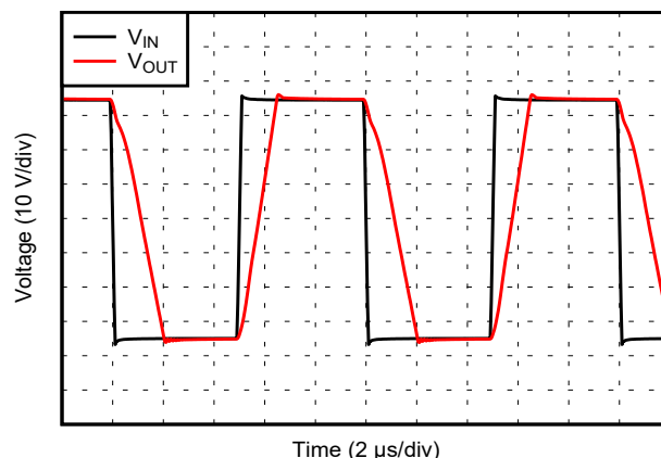
Figure 6-58. Large-Signal Step Response
