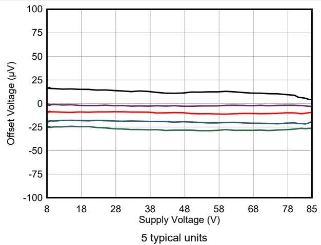
Figure 6-8. Input Offset Voltage vs Supply Voltage
