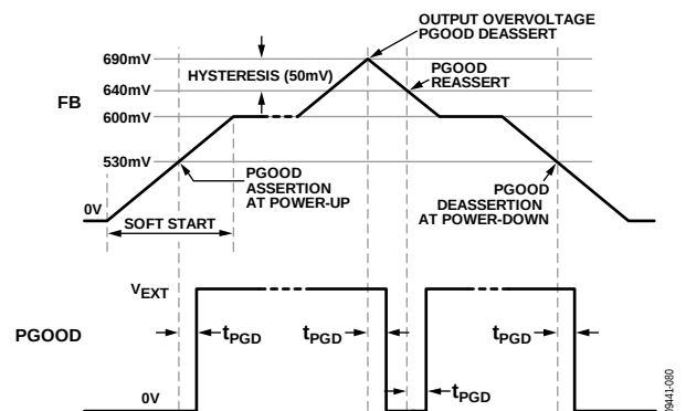
Figure 80. Power-Good Timing Diagram, t_{PG} = 12 \mu s (Diagram May Look Disproportionate For Illustration Purposes)
