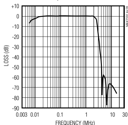
BASEBAND CHANNEL FREQUENCY RESPONSE
