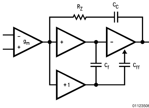
FIGURE 1. LMC6024 Circuit Topology (Each Amplifier)
