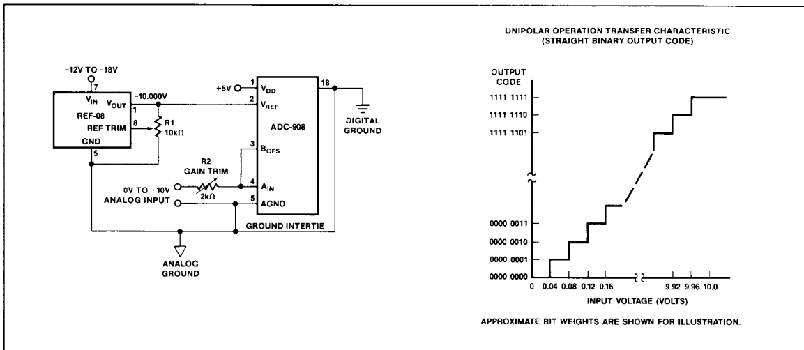
FIGURE 7: Unipolar Operation
