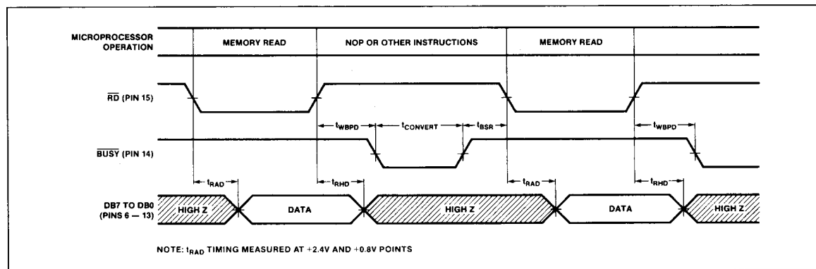
FIGURE 3: ROM Mode Timing Diagram ( \bar{CS} Held LOW)
