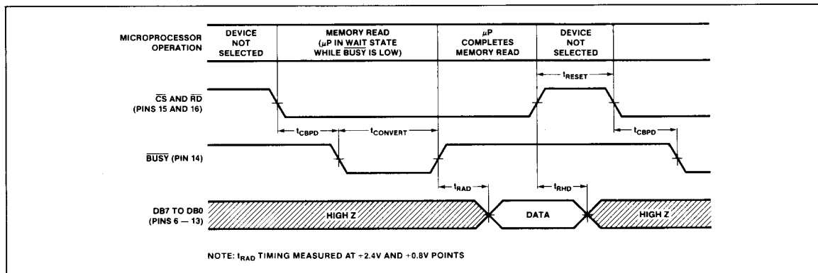
FIGURE 4: Slow-Memory Mode Timing Diagram ( \bar{CS} and \bar{RD} Tied Together)
