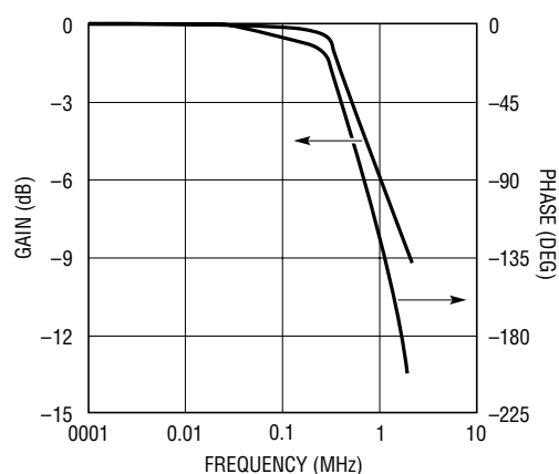
Differential Amplifier Gain-Phase
