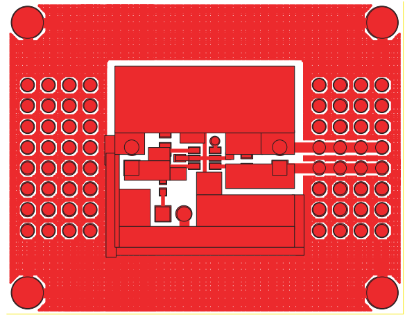
Figure 2: AAT4280 Evaluation Board Component Side Layout.
