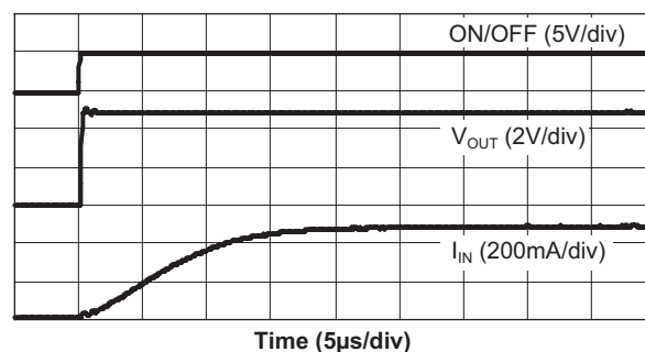
AAT4280-2 Turn-On ( V_{IN} = 5V ; R_L = 10\Omega )
