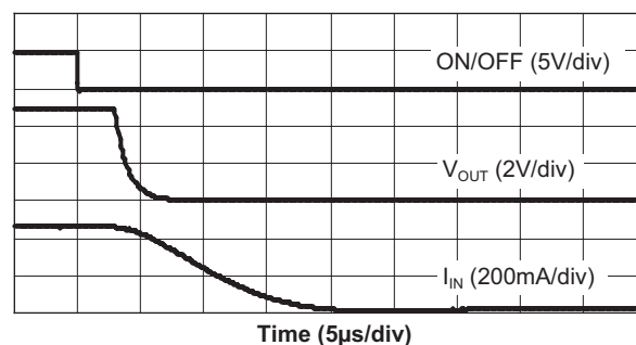
AAT4280-2 Turn-Off ( V_{IN} = 5V ; R_L = 10\Omega )
