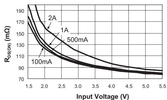
R_{DS(ON)} vs. Input Voltage
