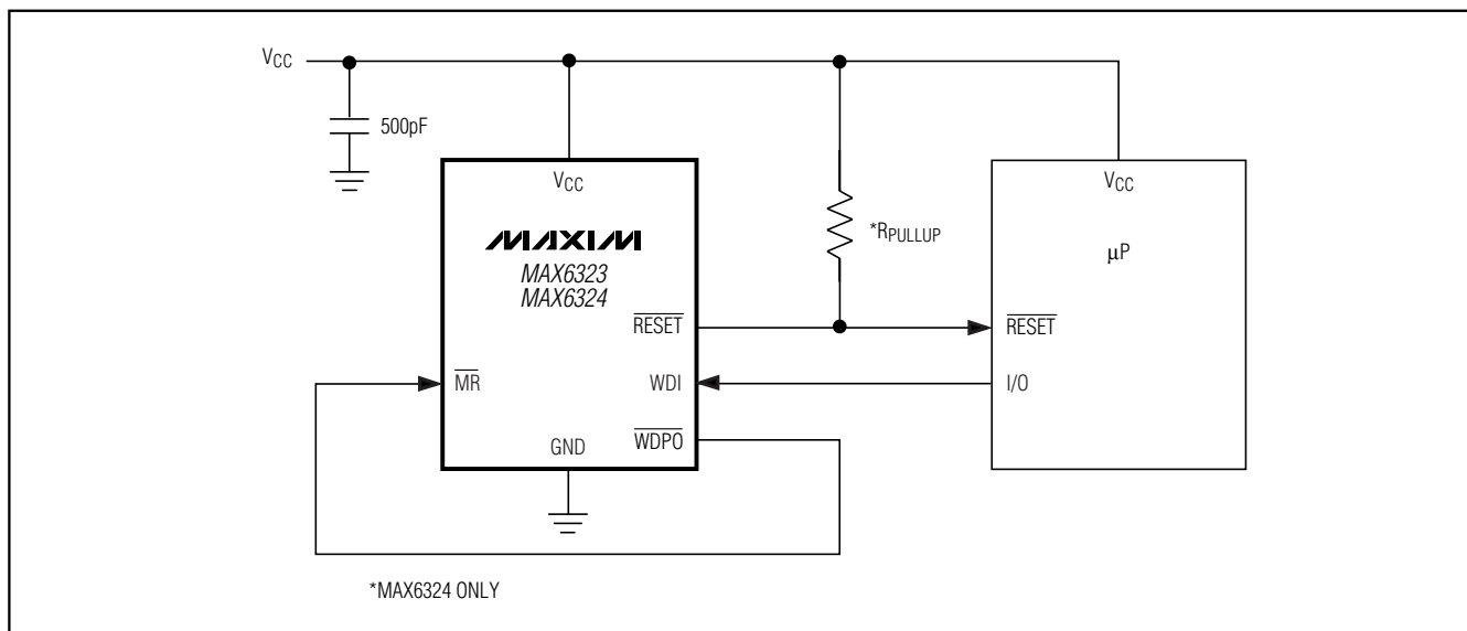
Figure 10. \overline{\text{WDPO}} to \overline{\text{MR}} Loopback Circuit
