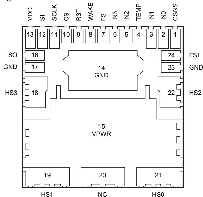
Figure 3. 33580 Pin Connections
