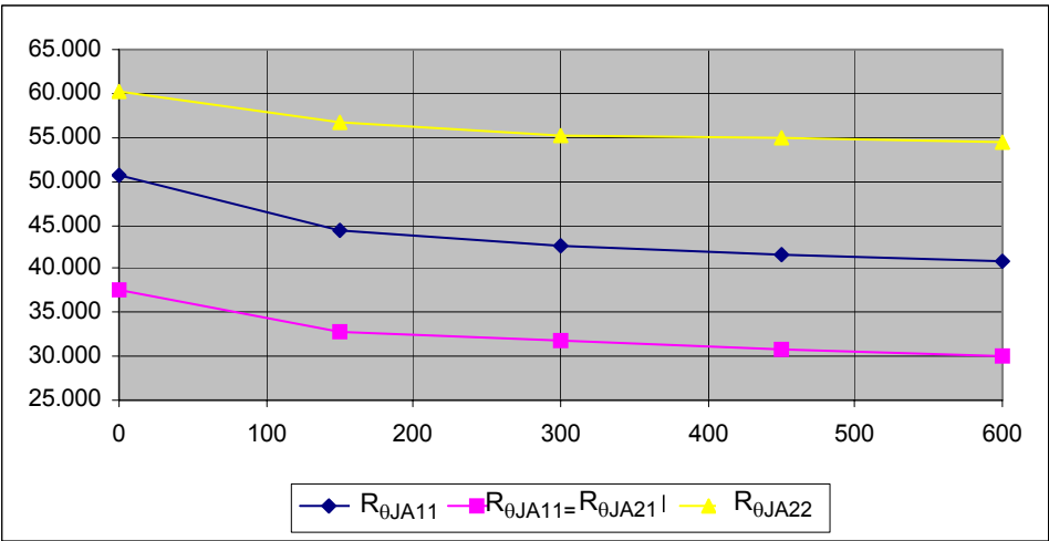
Figure 13. Stead State Thermal Resistance
