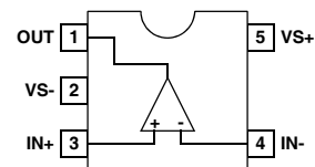
EL5192 (5 LD SOT-23) TOP VIEW
