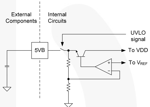
Figure 17. 5 V Bias
