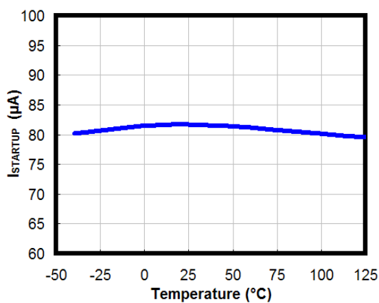
Figure 37. I_{\text{STARTUP}} vs. Temperature
