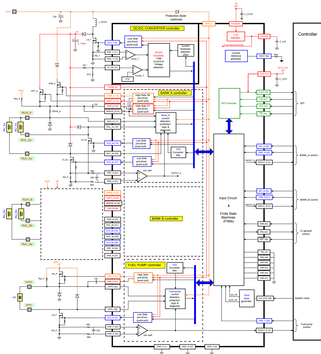
Figure 2. Block diagram
