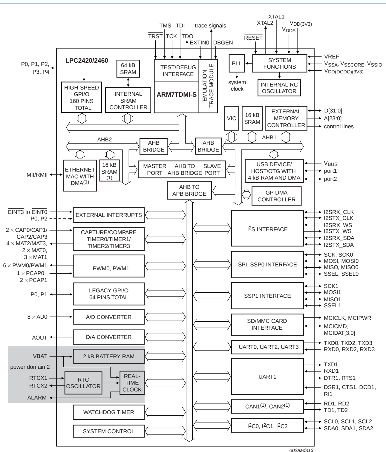
Fig 1. LPC2420/2460 block diagram
