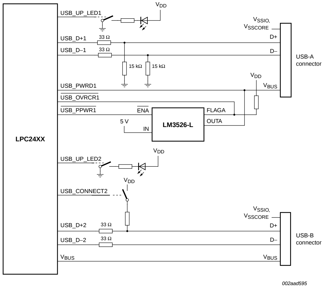
Fig 27. LPC2420/2460 USB OTG port configuration: USB port 2 device, USB port 1 host
