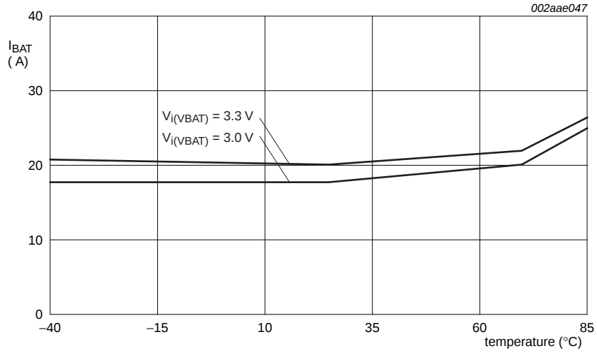
Fig 9. RTC battery maximum supply current I_{BAT} versus temperature in Deep power-down mode
