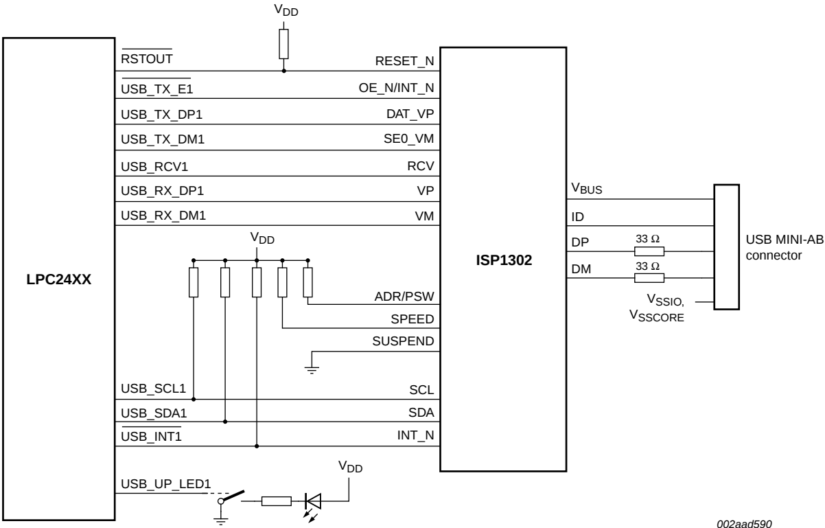
Fig 26. LPC2420/2460 USB OTG port configuration: VP_VM mode
