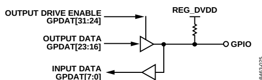
Figure 28. ADuC7039 GPIO
