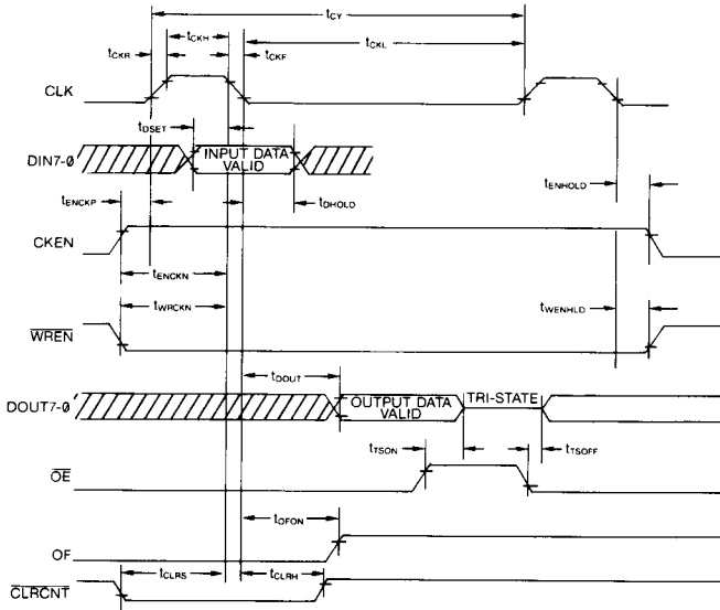
FIGURE 2: SINGLE ROW BUFFER READ TIMING
