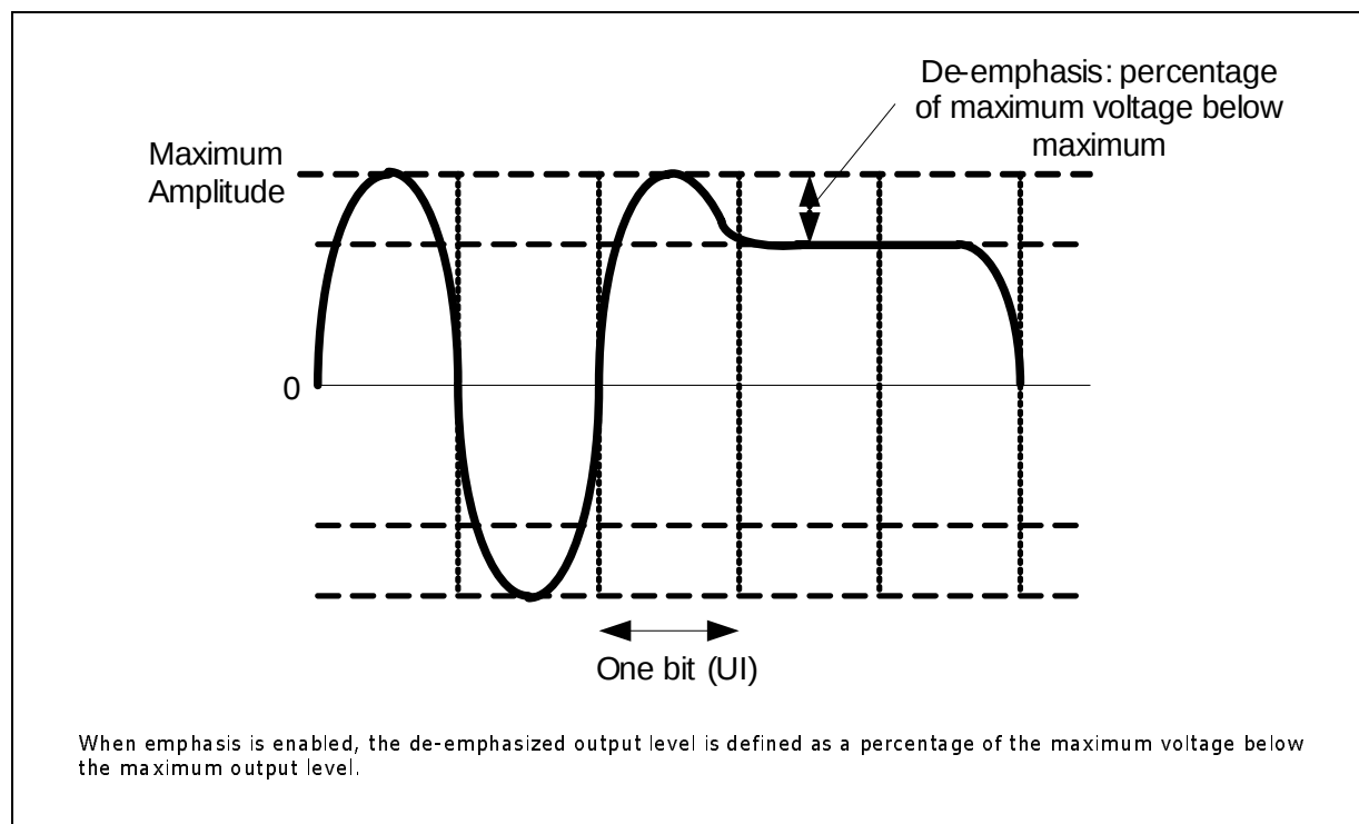
Figure 27. Maximum Amplitude
