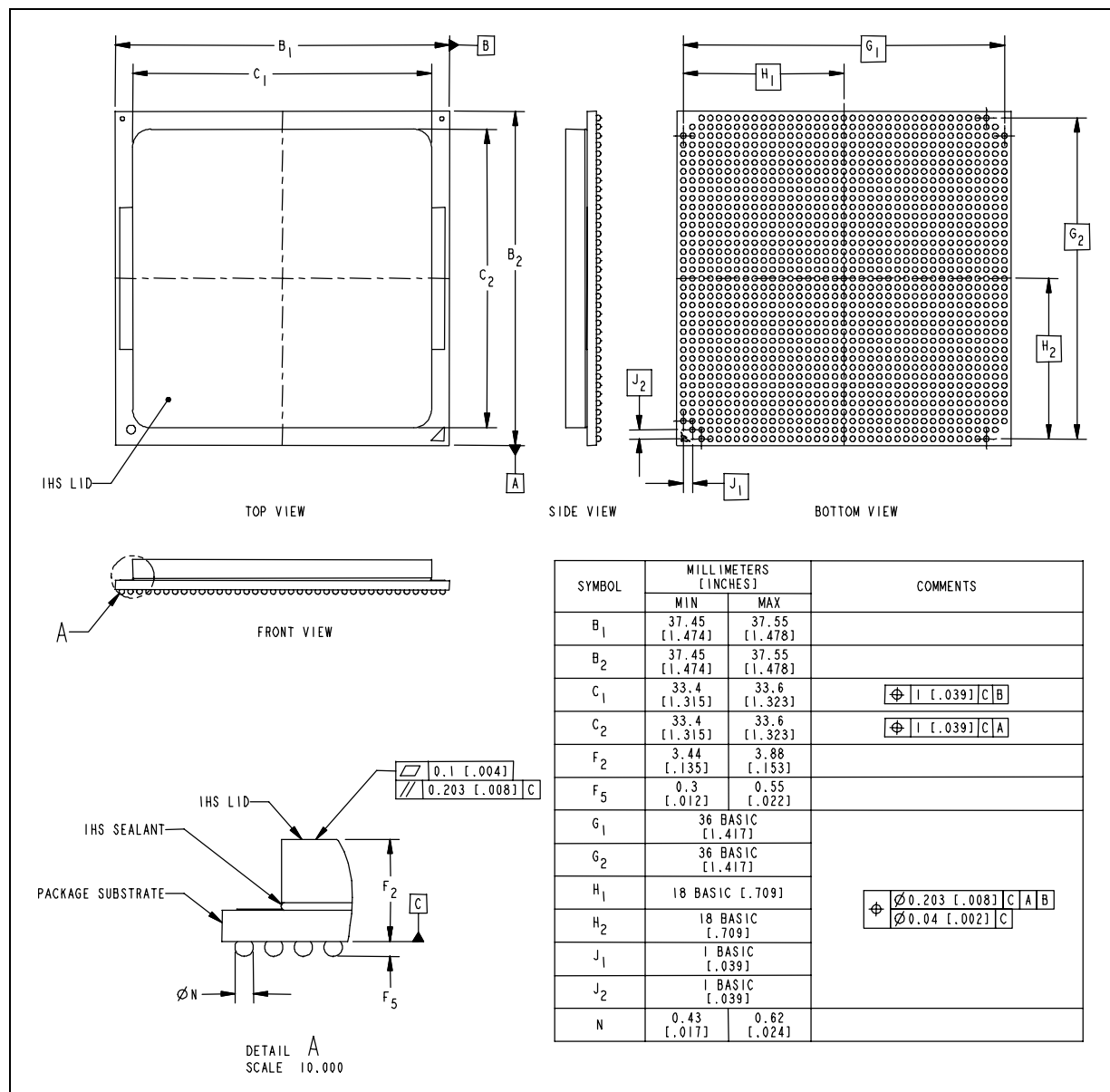
Figure 2. 1357-Lead FCBGA Package (Top and Bottom Views)
