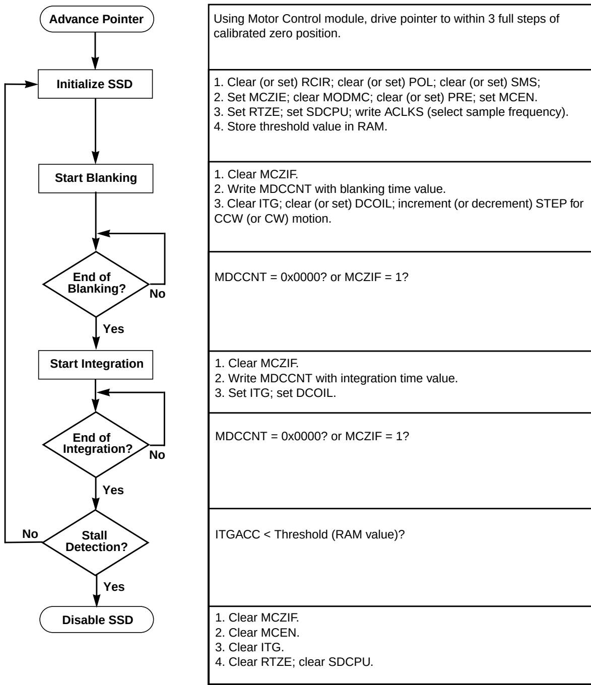
Figure 21-15. Return-to-Zero Flowchart
