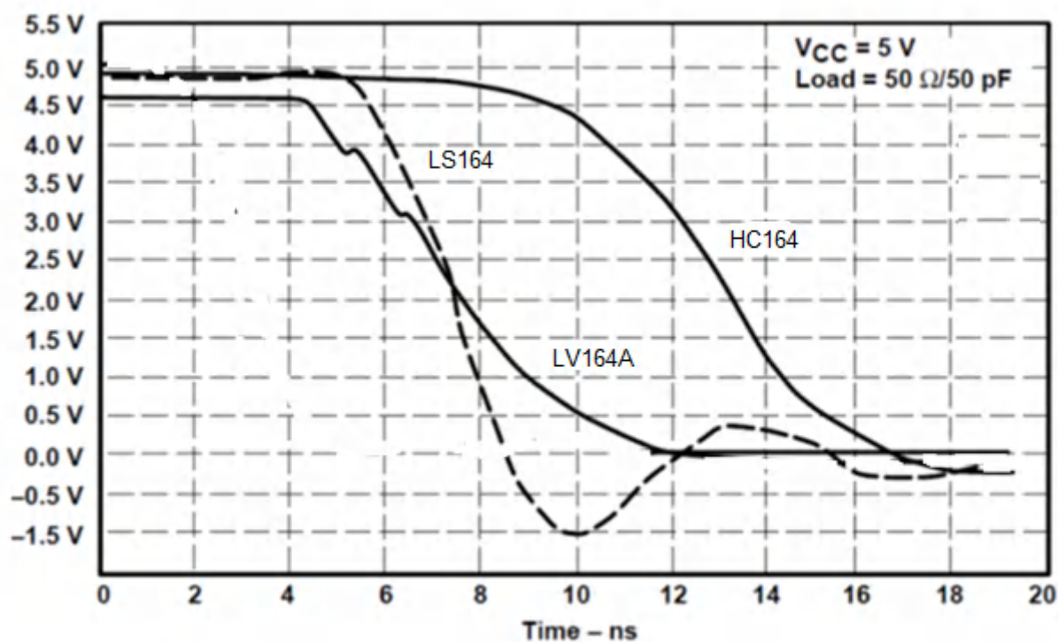
Figure 9-2. Switching Characteristics Comparison
