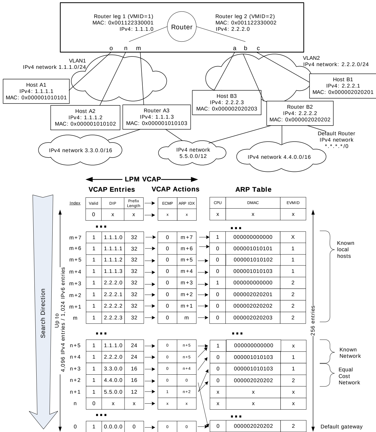
Figure 44 • IP Unicast Routing Example
