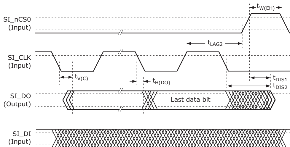
Figure 178 • SI Output Data Timing Diagram for Slave Mode
