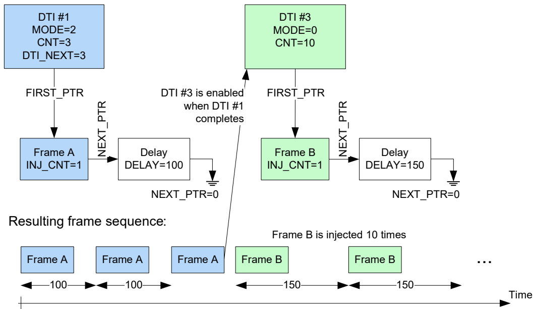
Figure 111 • DTI Concatenation
