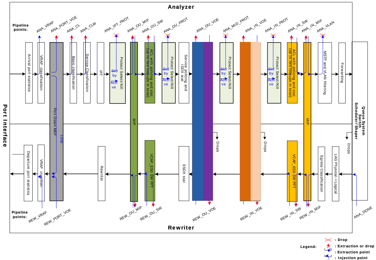
Figure 30 • Processing Flow
