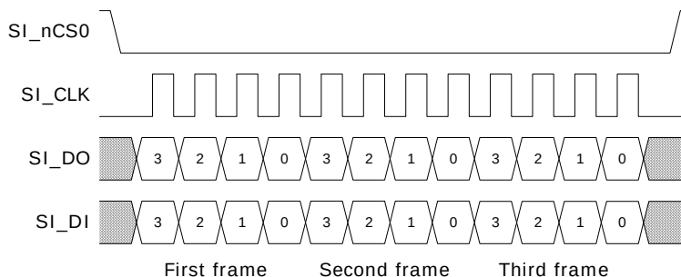
Figure 158 • SIMC SPI 3x Transfers
