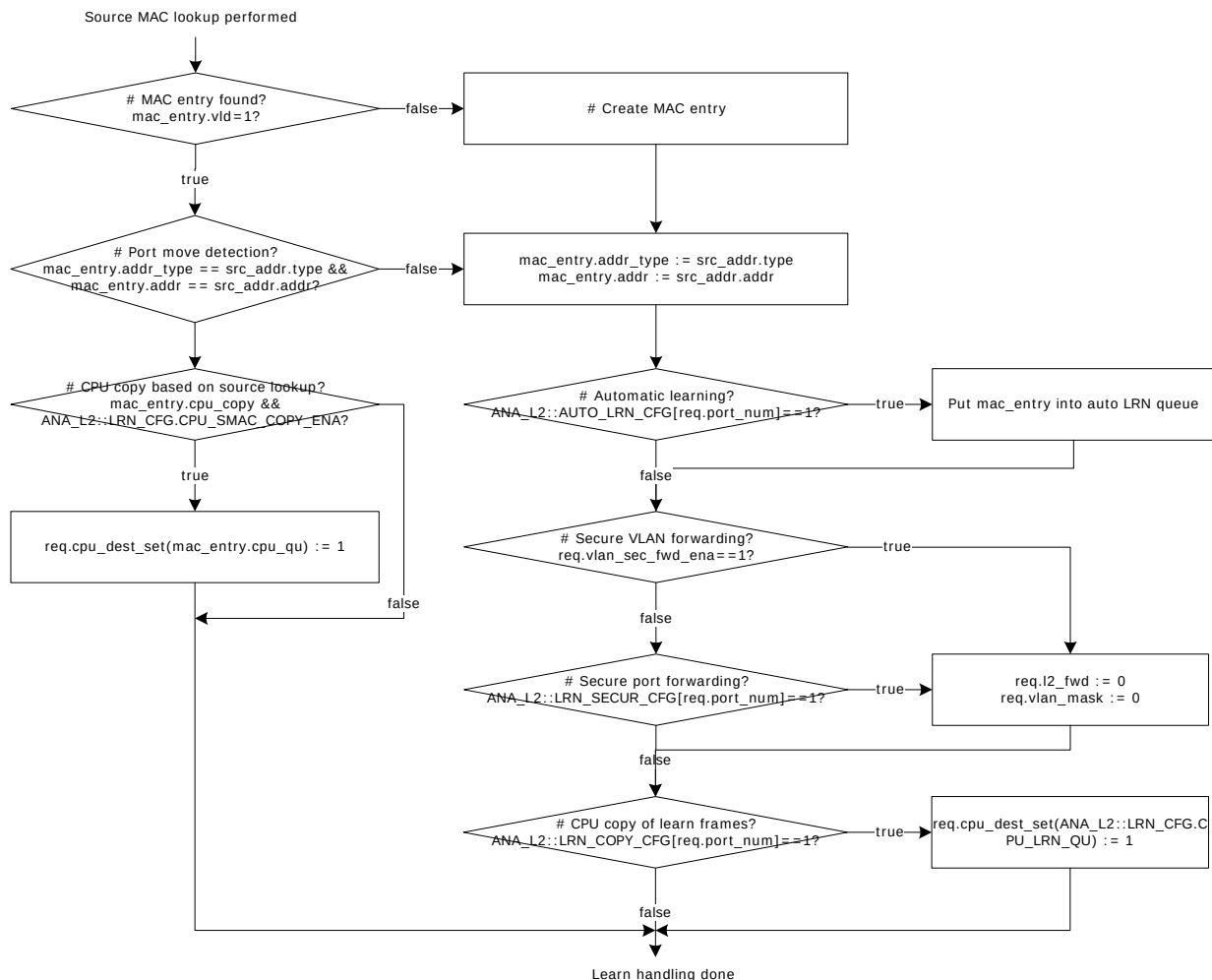
Figure 49 • Source Check
