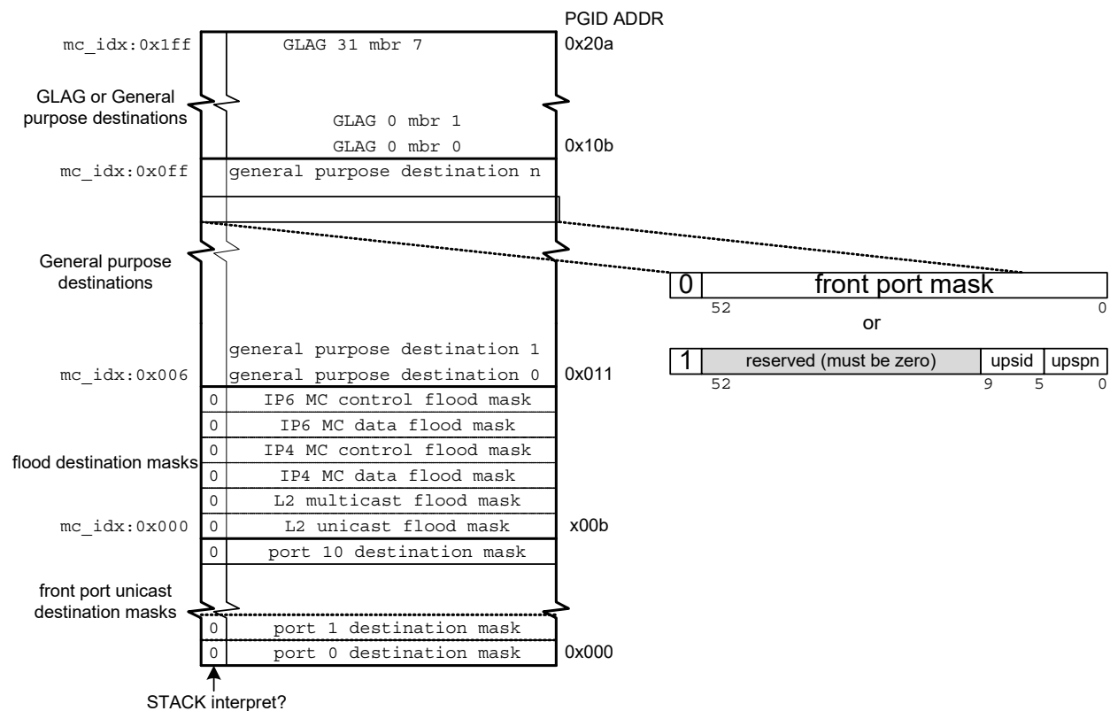
Figure 50 • PGID Layout
