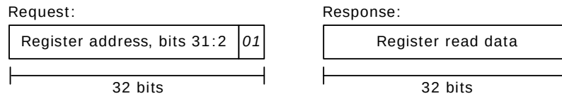
Figure 128 • WRITE Command
