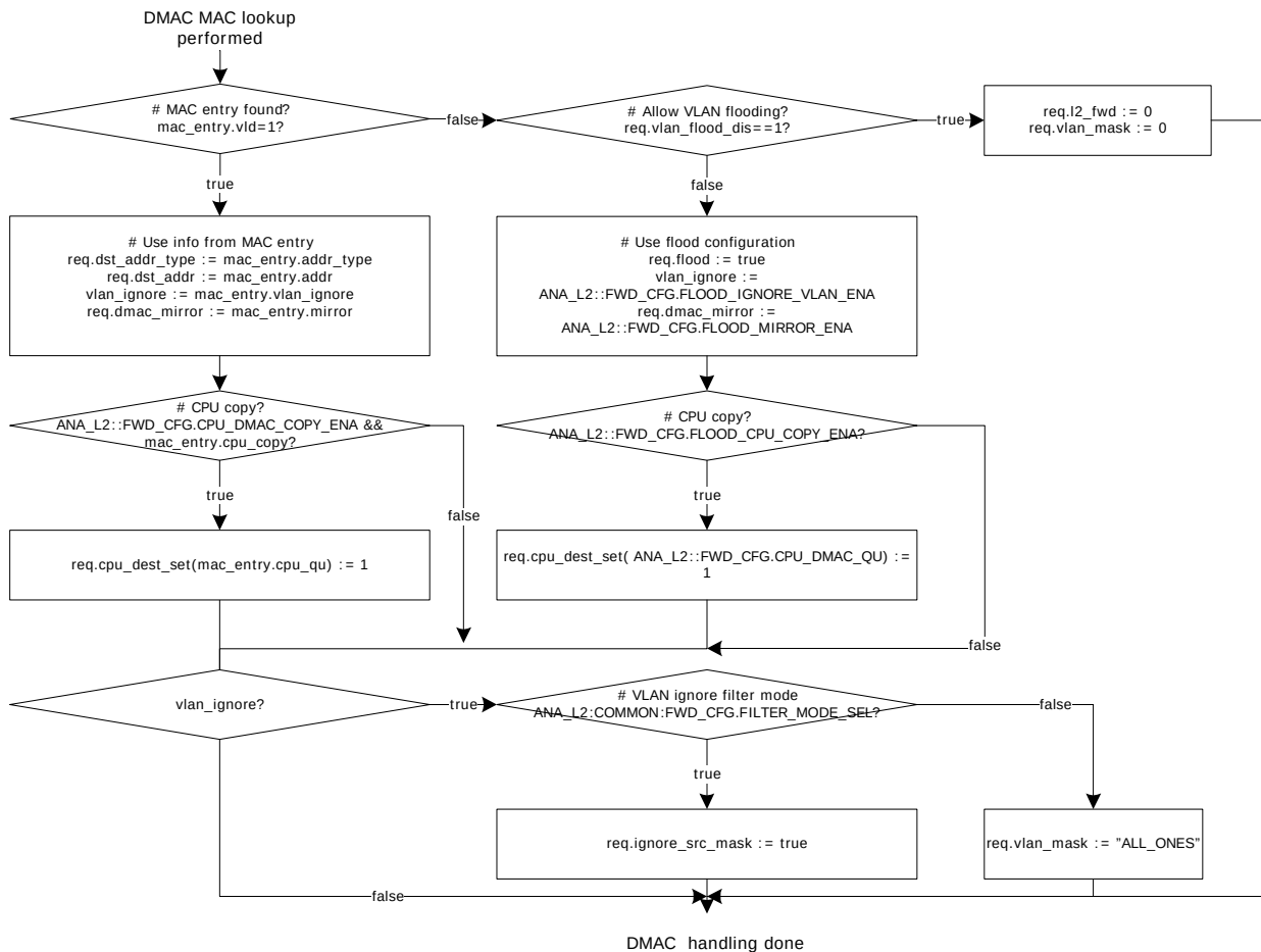
Figure 48 • DMAC Lookup
