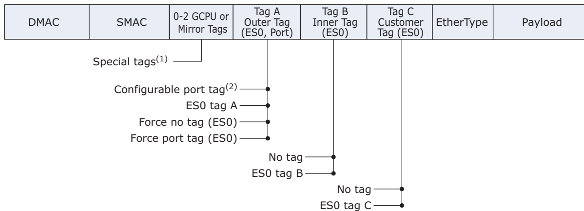
Figure 116 • VLAN Pushing
