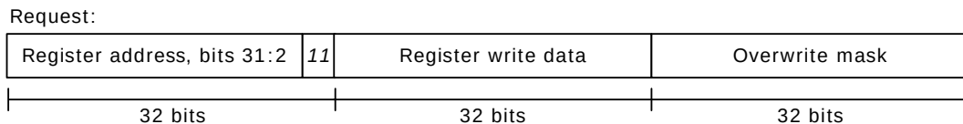
Figure 129 • READ-MODIFY-WRITE Command
