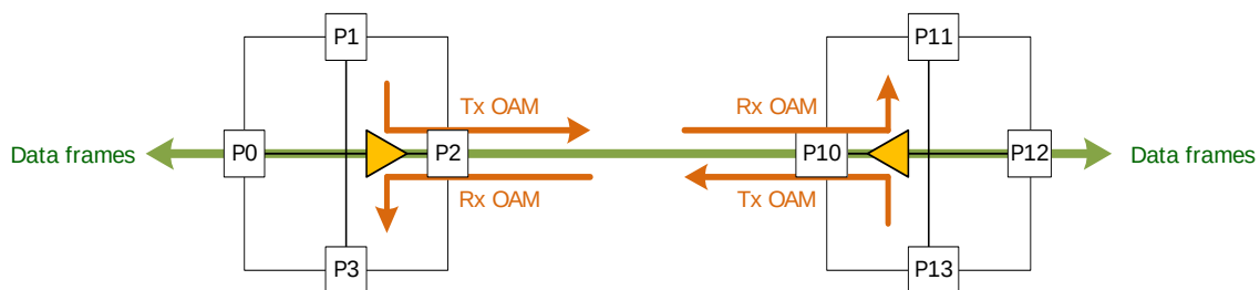
Figure 65 • Down-MEP Location
