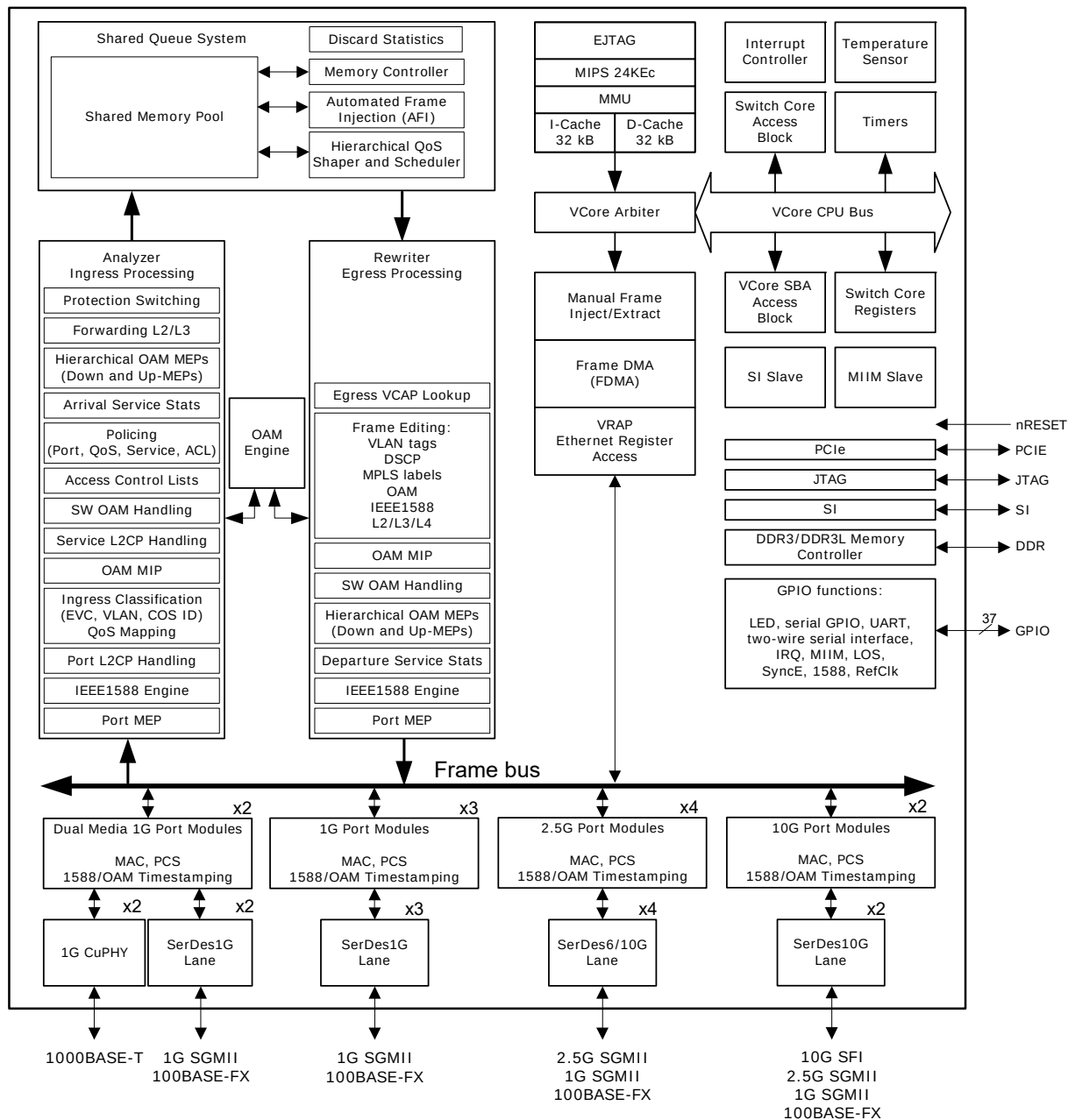
Figure 10 • Block Diagram
