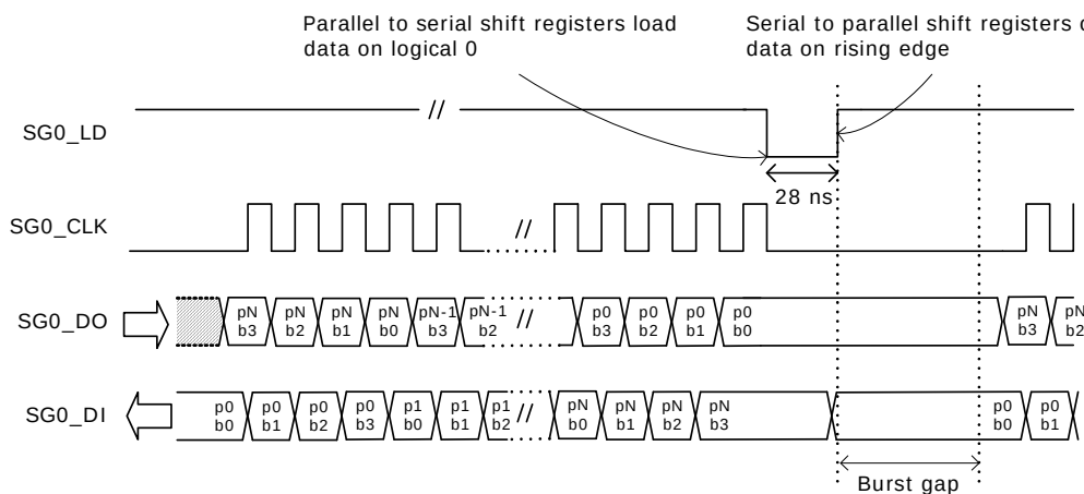
Figure 163 • SIO Timing
