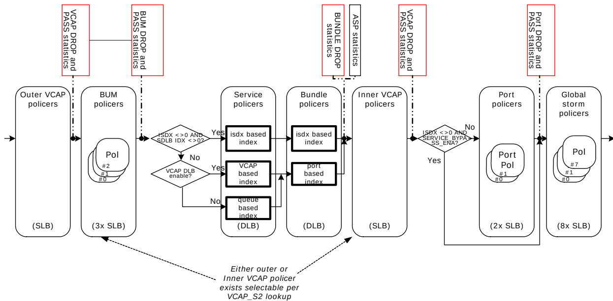
Figure 54 • Policer Hierarchy
