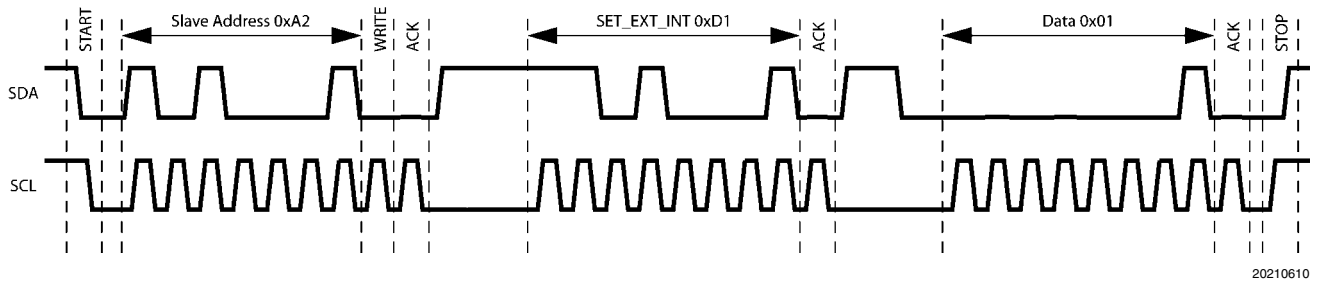
FIGURE 8. Host Write Command
