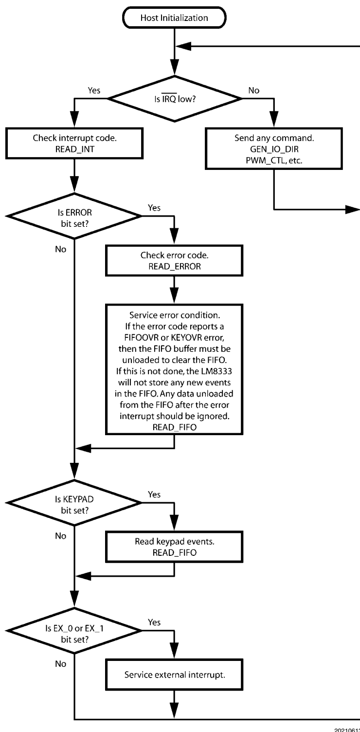
FIGURE 11. Interrupt Processing
