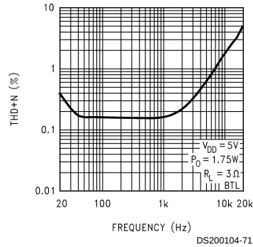
LM4840MH, LM4840LQ THD+N vs Frequency
