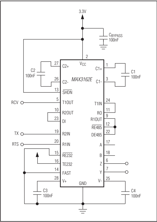
Figure 18. Protocol Translator
