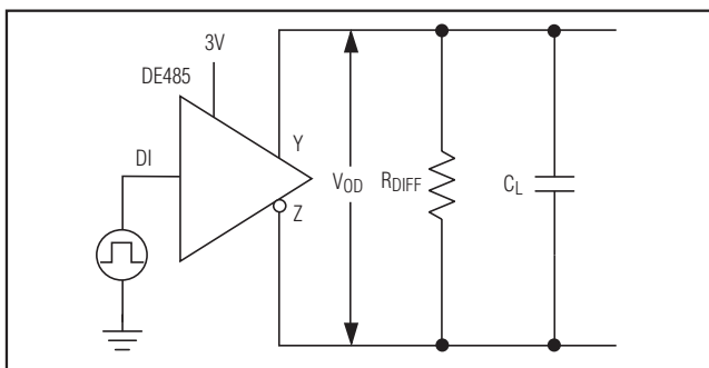
Figure 3. RS-485/RS-422 Driver Timing Test Circuit
