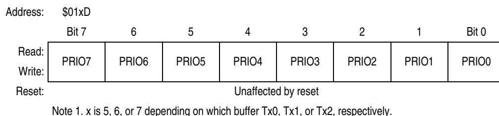
Figure 16-15. Transmit Buffer Priority Register (TBPR)
