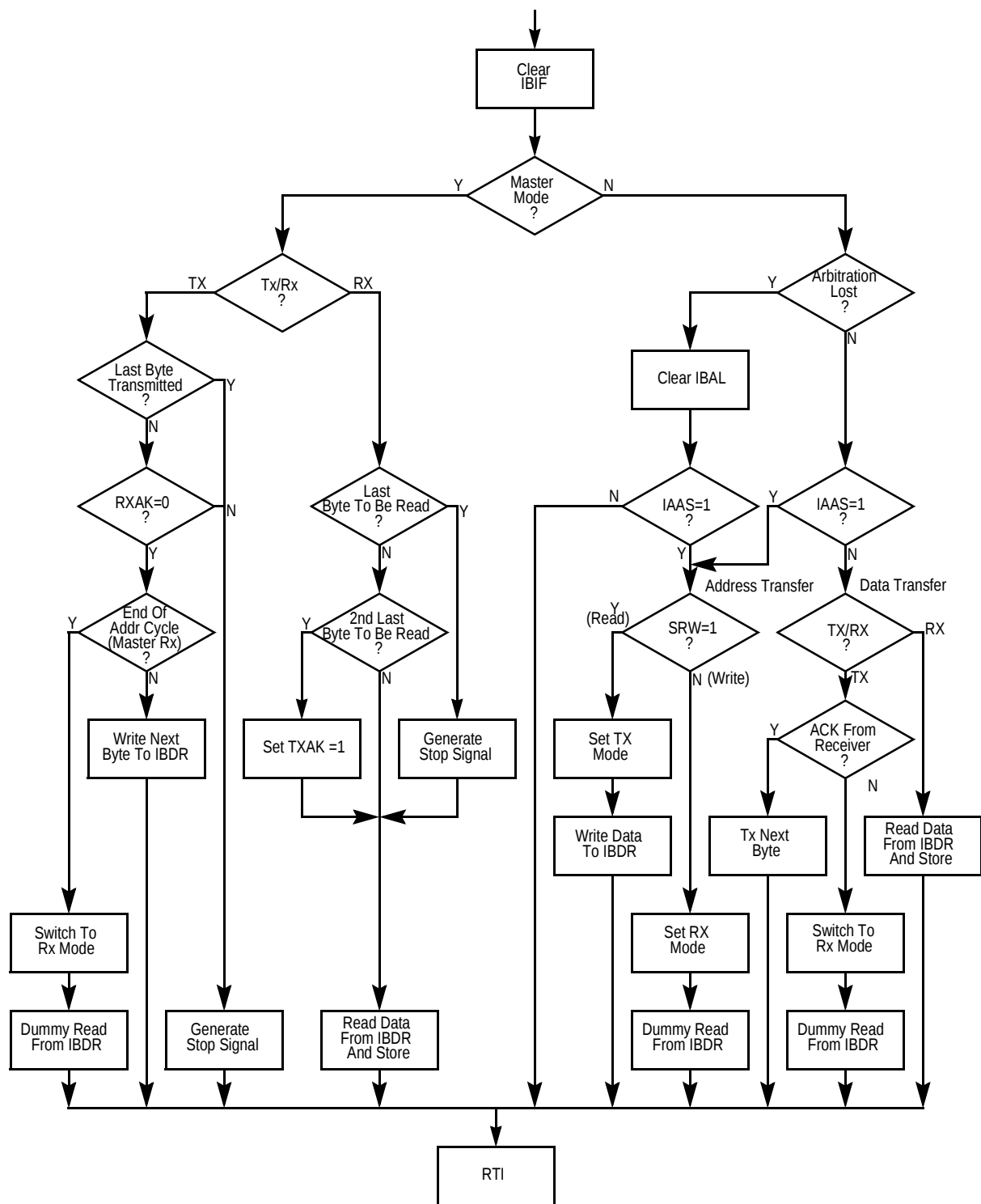
Figure 40 Flow-Chart of Typical IIC Interrupt Tx Routine
