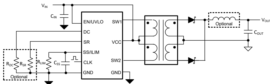
Simplified Schematic
