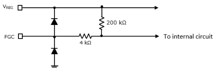
Internal circuit diagram of FGC pin
