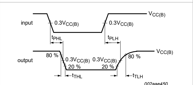
Figure 16. Propagation delay and transition times; CEC in to CEC out
