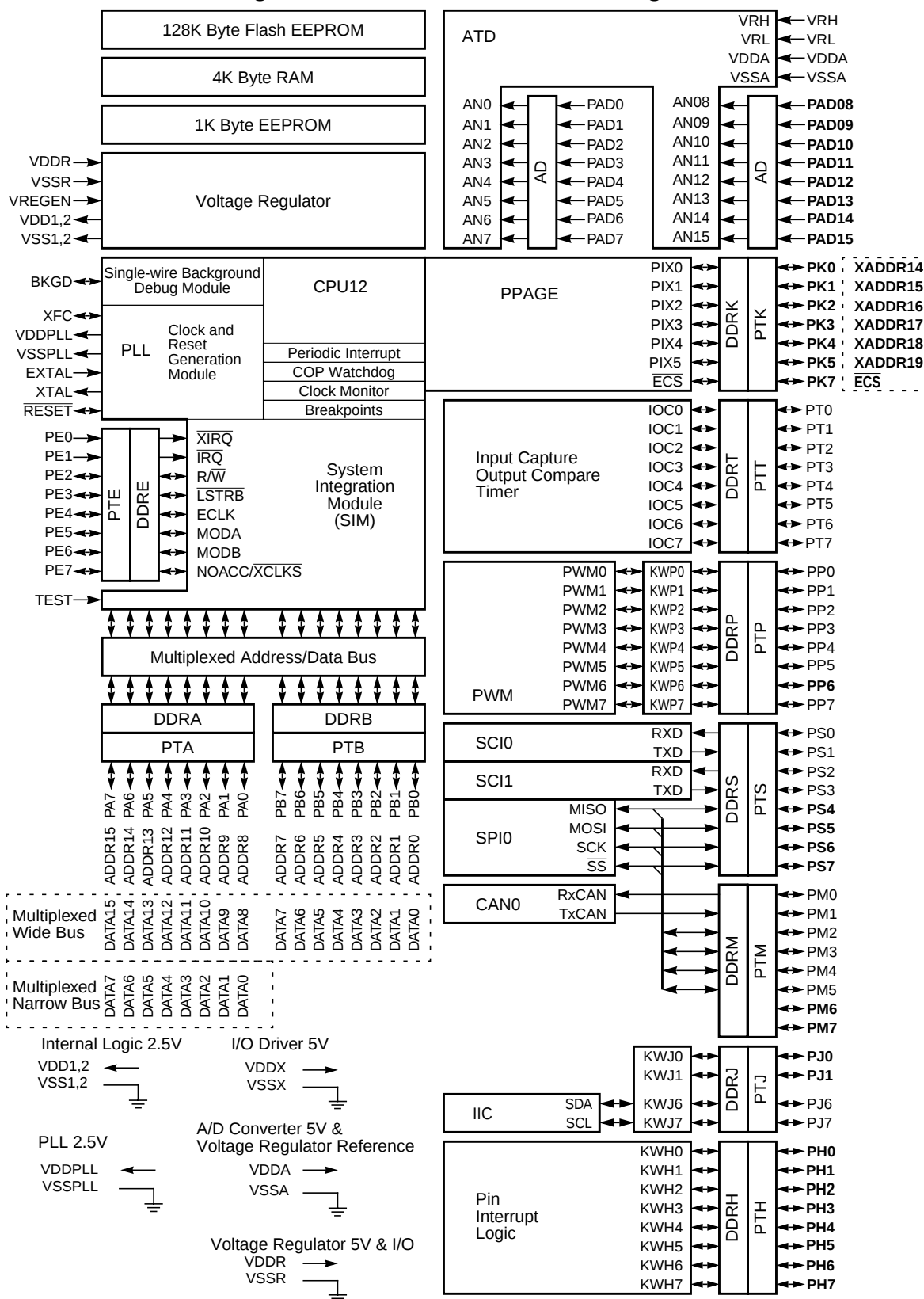
Figure 1-1 MC9S12B128 Block Diagram
