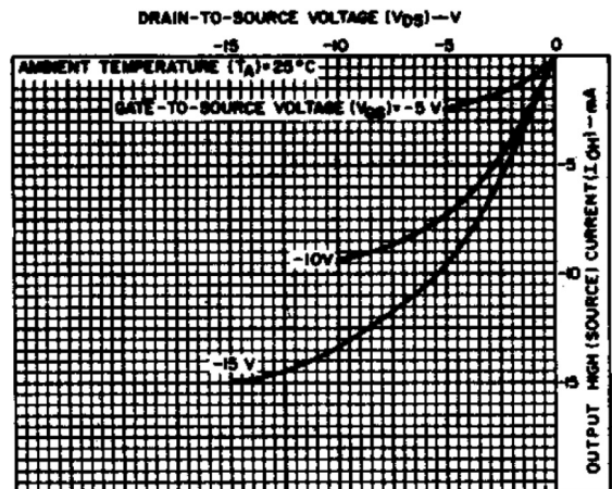
Figure 4. Minimum Output High (Source) Current Characteristics
