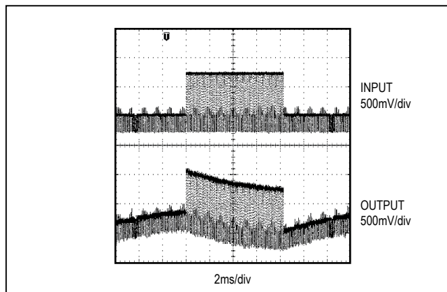
Figure 1. AC-Coupled Output
