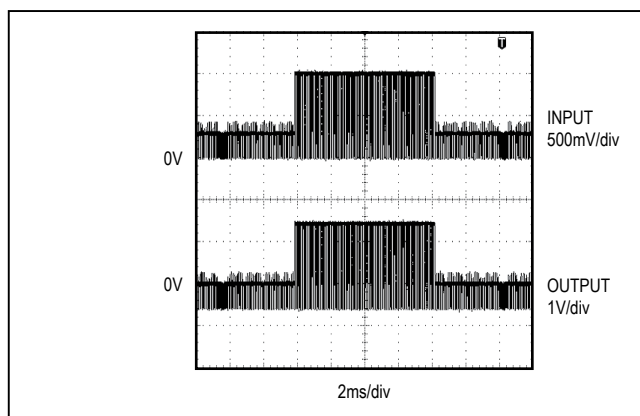
Figure 2. DirectDrive Output
