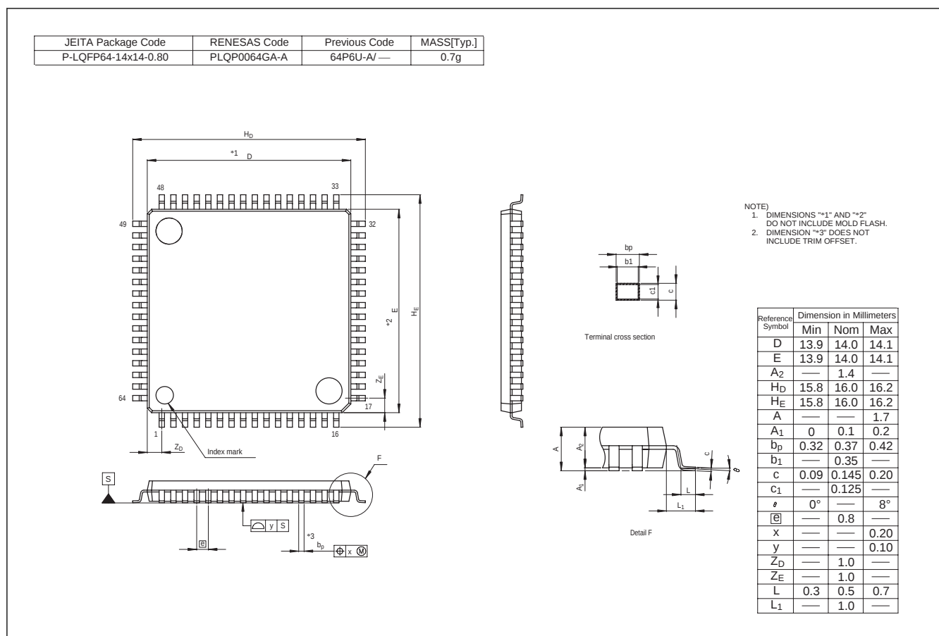
Figure 2.3 LQFP 64-pin
