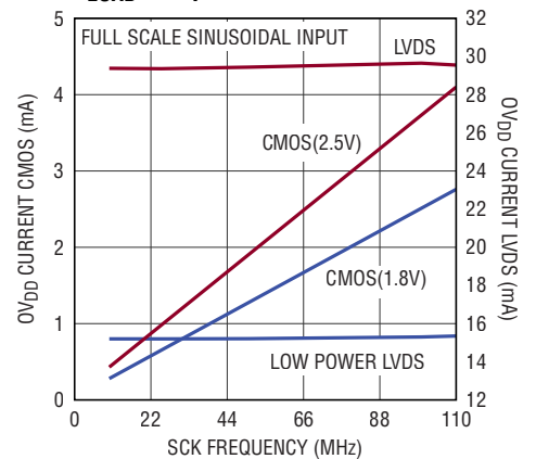
0V_{DD} Current vs SCK Frequency, C_{\text{LOAD}} = 10\text{pF}
