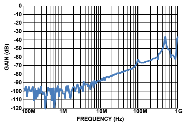
FIGURE 38. CHANNEL-TO-CHANNEL X-TALK
