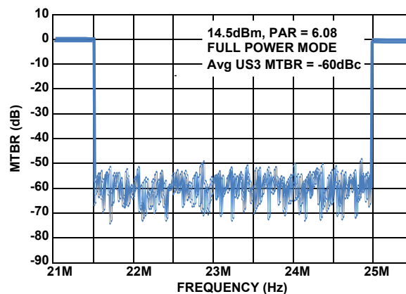
FIGURE 32. VDSL2 30a PROFILE MTBR US3
