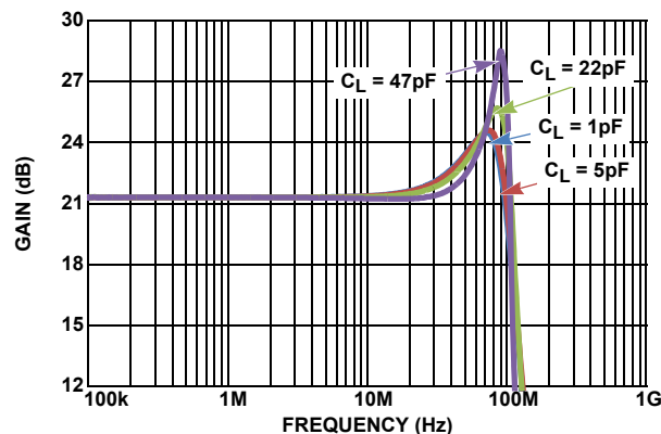
FIGURE 28. SMALL SIGNAL FREQUENCY RESPONSE vs C_{LOAD} (AFTER RB)
