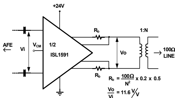
FIGURE 1. FIXED GAIN LINE DRIVER CIRCUIT
