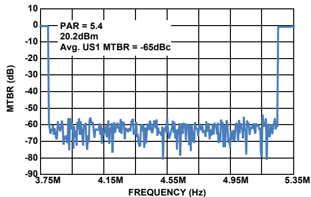
FIGURE 36. VDSL2+ 8b PROFILE MTBR
