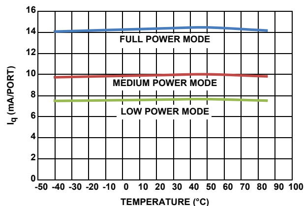
FIGURE 43. QUIESCENT CURRENT vs TEMPERATURE
