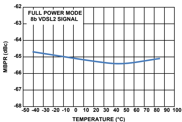
FIGURE 45. 8b MBPR vs TEMPERATURE
