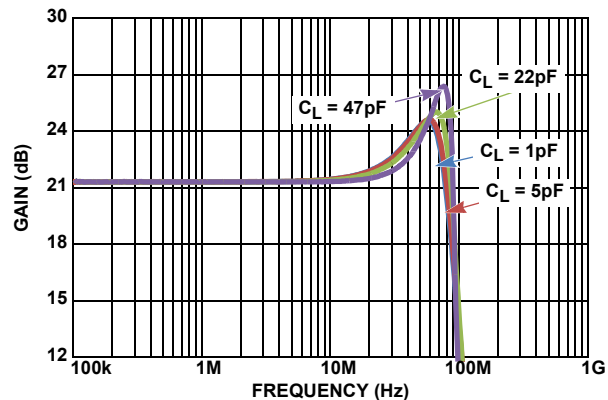
FIGURE 34. SMALL SIGNAL FREQUENCY RESPONSE vs C_{LOAD}
