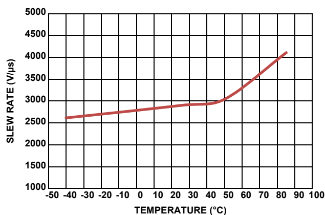
FIGURE 47. SLEW RATE vs TEMPERATURE
