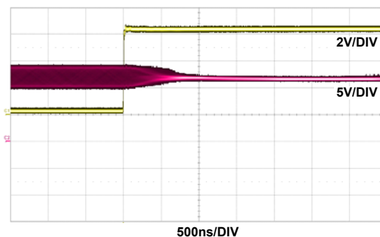
FIGURE 40. POWER-DOWN TIME
