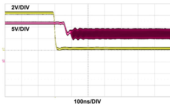
FIGURE 39. POWER-UP TIME
