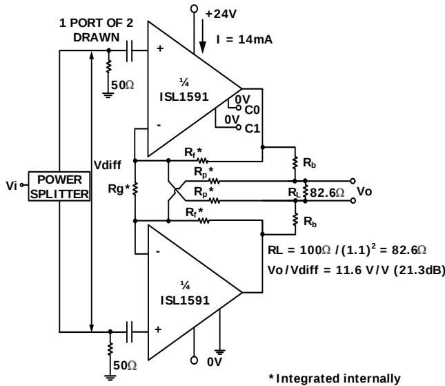
FIGURE 49. ACTIVE TERMINATION TEST CIRCUIT
