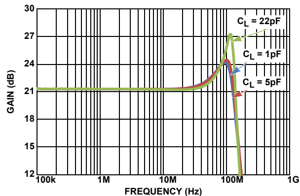
FIGURE 23. SMALL SIGNAL FREQUENCY RESPONSE vs C_{LOAD} (AFTER R_b )
