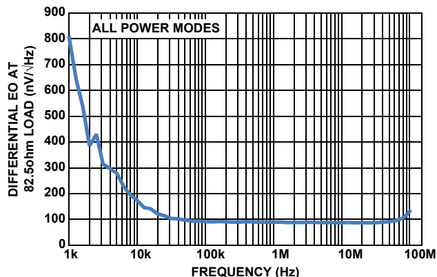
FIGURE 25. OUTPUT VOLTAGE NOISE
