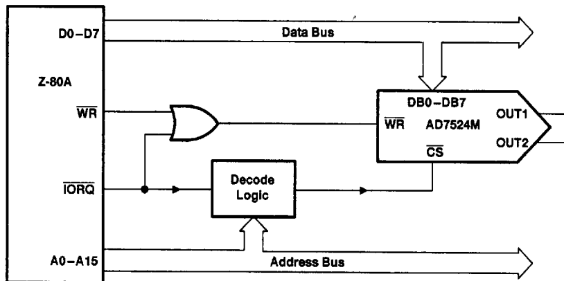
Figure 4. AD7524M-Z-80A Interface
