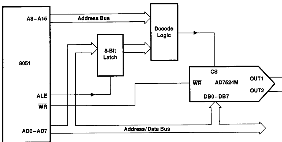
Figure 6. AD7524M-8051 Interface
