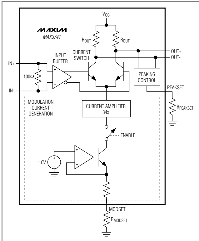
Figure 2. Modulation Circuit
