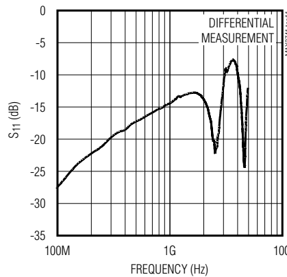
INPUT RETURN LOSS
