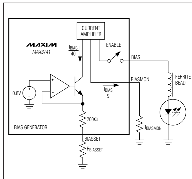
Figure 1. Bias Generator
